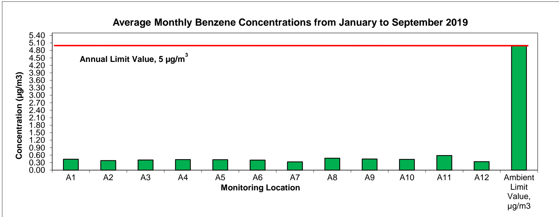
Figure 3 Average Monthly Benzene ( \text{C}_6\text{H}_6 ) Concentrations Q3 2019
