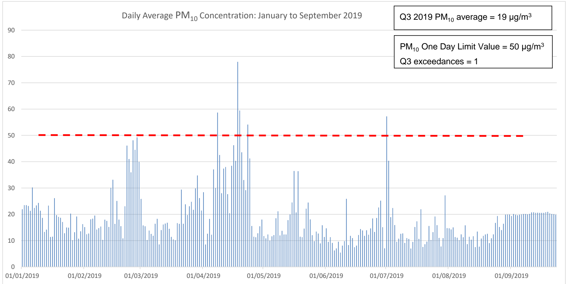
Figure 5 Daily Average PM 10 Q3 2019
